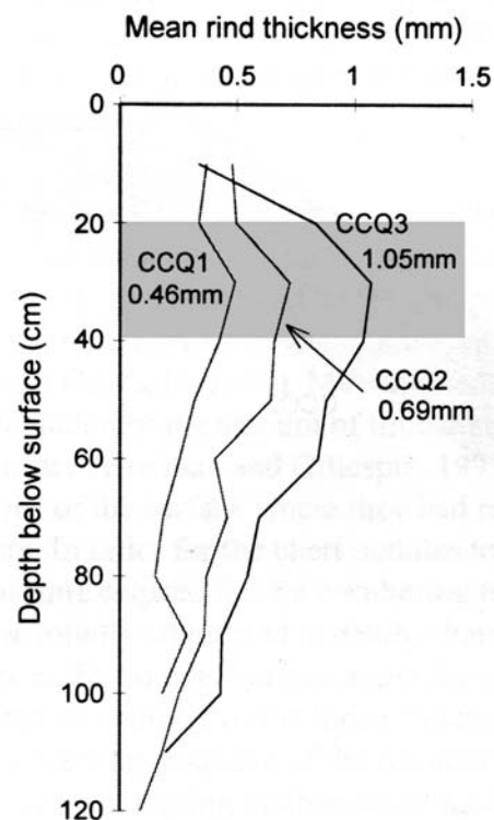
Figure 3.5. Plots of the mean carbonate rind thickness on clasts at depth in three Cottonwood Canyon surfaces. The rind thickness increases to a maximum at relatively shallow depth for each surface. The maximum thickness increases with surface age (CCQ1 is the youngest, CCQ3 is the oldest), which is the basis for the chronosequence shown in Fig. 3.6. The mean rind thickness over the 20 cm interval where rinds are thickest (gray box) is given for each plot. See Fig. 3.3 for location of the surfaces and Stenner (1998) for raw data. Each rind thickness measurement has an uncertainty of \pm 0.02 mm.
