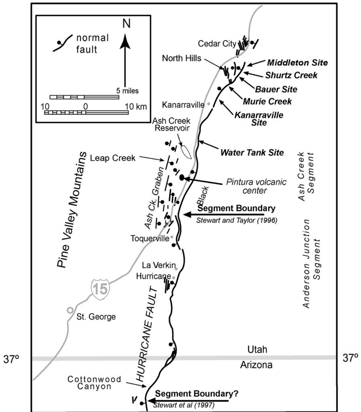
Figure 2.3. Hurricane fault in southwestern Utah showing sites with scarps on unconsolidated deposits; segment boundary of Stewart and Taylor (1996) shown with large arrow. Ash Creek graben and the Pintura volcanic center are also shown.
