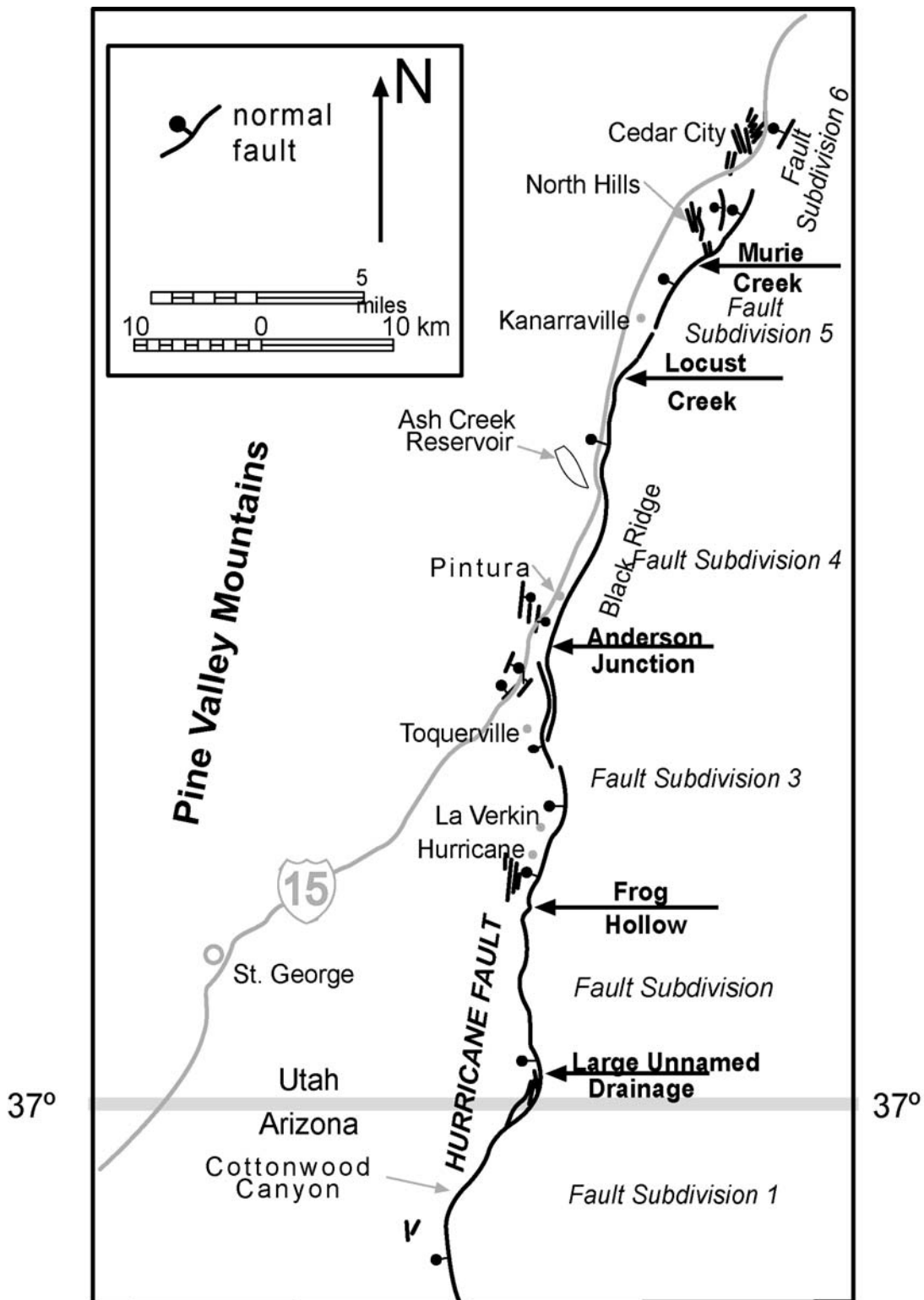
Figure 2.1. Hurricane fault and subsidiary structures in southwestern Utah. Fault subdivision boundaries defined for this study are delineated horizontal lines with arrows.
