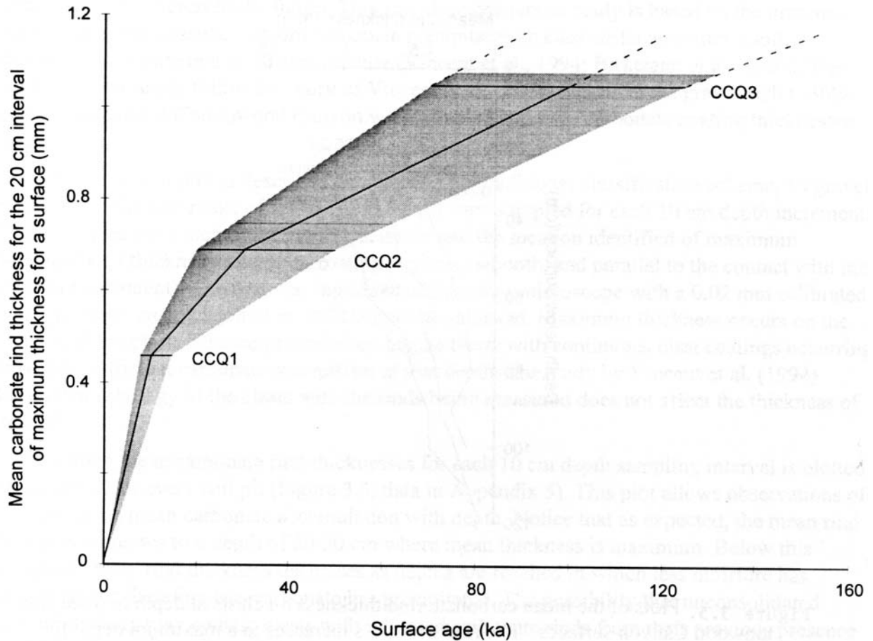
Figure 3.6. Soil chronosequence plot of the mean carbonate rind thickness (of the maximum 20 cm interval of the soil profile) and surface ages based on soil development and cosmogenic dating. The relationship shown in the plot allows future surface ages to be estimated using rind thickness. Uncertainty in the surface ages causes the grayed width to the relationship curve, with the preferred curve shown as a solid line.
