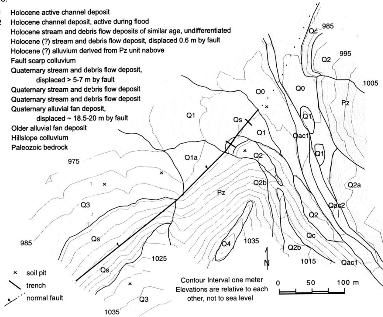
Figure 3.3. Quaternary geology and topography of the Cottonwood Canyon site, Arizona. Relationships between different-aged fault scarps, locations of trenches across the Hurricane fault, and soil pit locations are shown. The trend is for alluvial units to be older and higher in elevation away from the active channel and young alluvium commonly has buried the down-faulted portion of older units.
