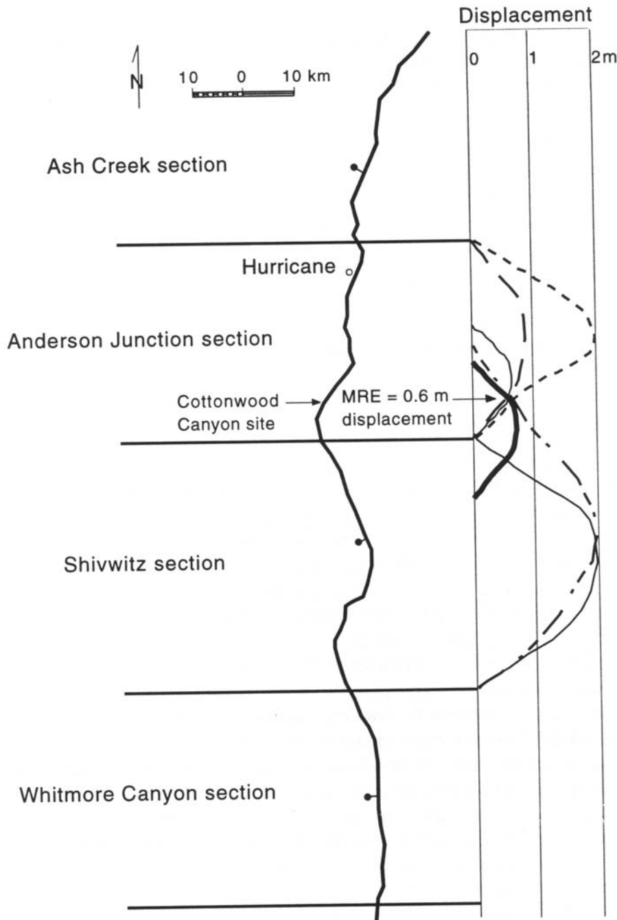
Figure 3.13. Possible rupture scenarios for the most recent event (MRE) recorded at the Cottonwood Canyon site where 0.6 m of vertical displacement occurred. Each MRE rupture is consistent with the amount of displacement evident from other scarp sites along the Anderson Junction section. Represented are a small magnitude rupture on the Anderson Junction section (long-dashed line), a small magnitude rupture across the section boundary (heavy solid line), a larger rupture on the Anderson Junction section (short-dashed line), a large rupture on the Shivwitz section that leaks north of the section boundary (dash-dot line), and a large rupture on the Shivwitz section that triggers a small event on the southern Anderson Junction section (thin solid line).
