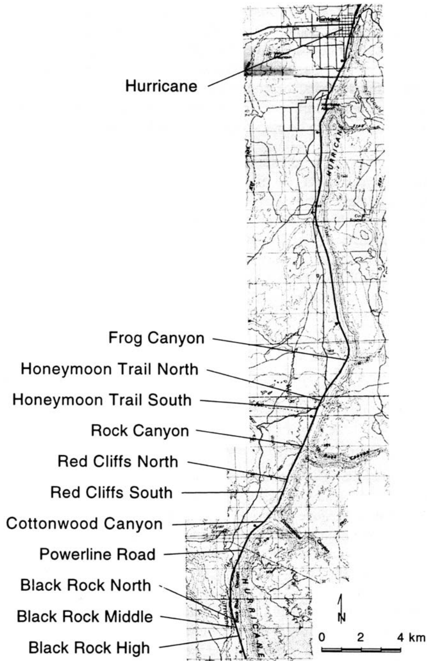
Figure 3.2. Topographic map of the study area within the Anderson Junction of the Hurricane fault. Locations of sites containing late Quaternary fault scarps discussed in the text are shown. Countour interval of the topographic base is 50 m (USGS, 1980, 1987). The fault is dashed where it is inferred (in the north where evidence for late Quaternary slip is not preserved and in the south where the location of the MRE is uncertain). The bar and ball are located on the down-thrown side of the fault.
