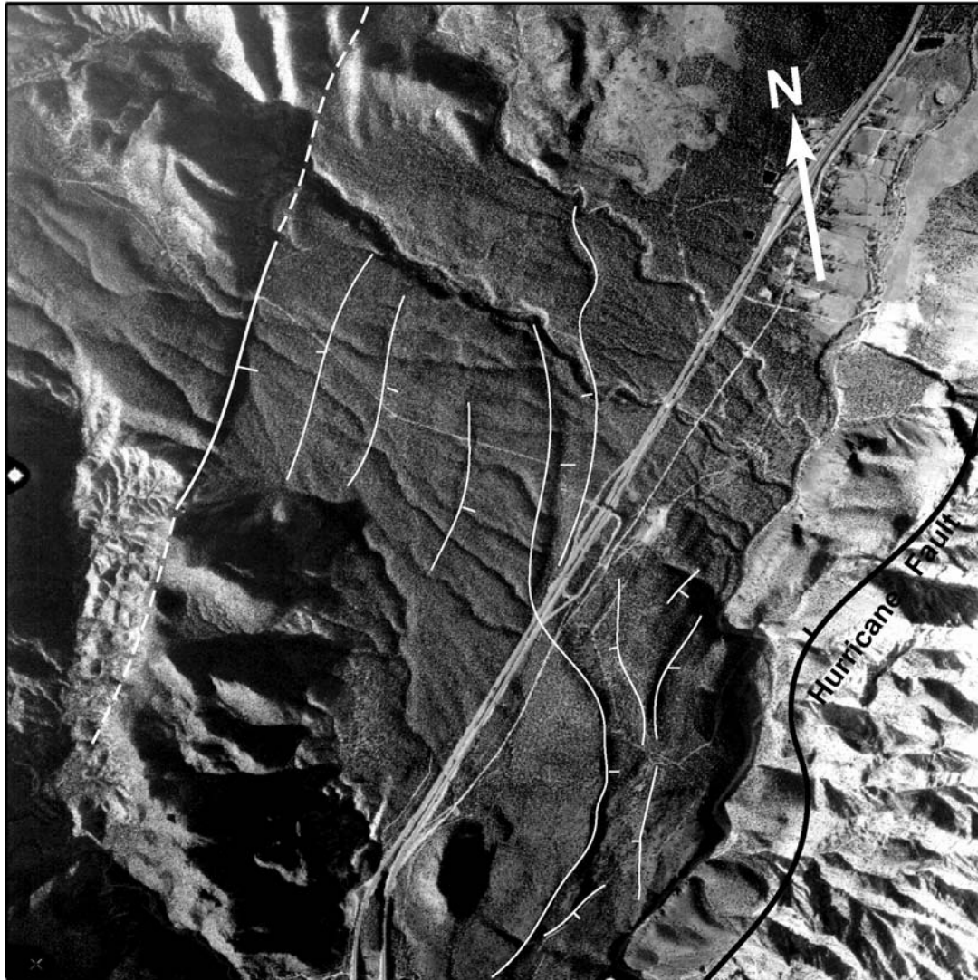
Figure 2.6. Oblique aerial view of the Hurricane fault (black) and antithetic and sympathetic faults (white) at the south end of the Ash Creek graben near Anderson Junction.
