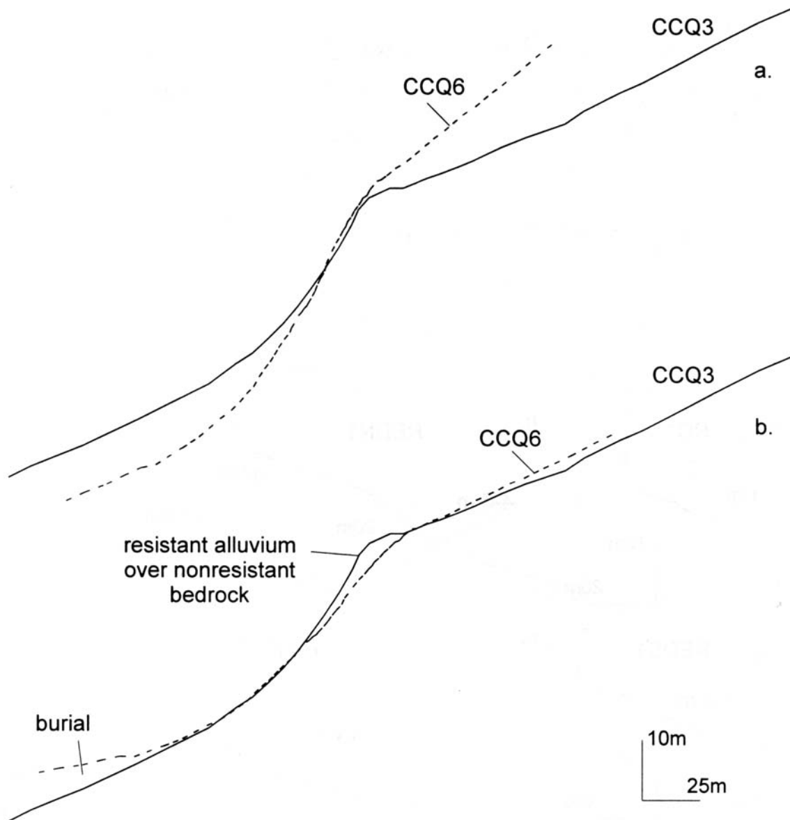
Figure 3.10. Topographic profiles of the Cottonwood Canyon alluvial fan fault scarps CCQ3 and CCQ6. In (a) the profiles are shown in their original surveyed form, with vertical exaggeration. Notice that the CCQ6 landform has a steeper overall slope. In (b) CCQ6 has been rotated to show that the two scarps have a similar shape and similar displacements. The close relationship between these two scarps forms the basis for using surface ages estimated for CCQ3 for CCQ6 as well. Differences between the two landforms exist at the base of the scarps, where CCQ6 has been buried by younger material that was noted in the field, and at the crests where CCQ3 exposes resistant alluvium over nonresistant bedrock causing a steepened slope.
