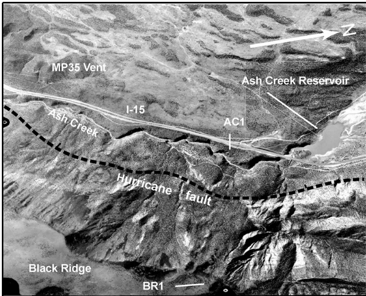
Figure 2.8. Oblique aerial view of the Pintura volcanic center showing the location of the MP35 vent and ^{40}\text{Ar}/^{39}\text{Ar} isotopic sample locations BR1 and AC1.8.
