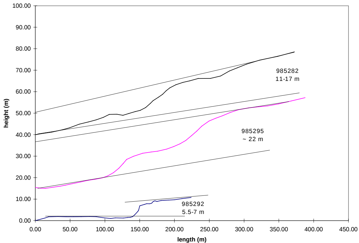
Figure 4.4. Representative topographic profiles across the Hurricane fault on the ~100 ka Bar Ten basalt flow. The surface of the basalt flow is quite irregular so projection of surfaces across the fault zone is fraught with uncertainty. We suspect that the bottom profile does not capture all of the late Quaternary displacement because of multiple fault strands. The middle profile may capture some topographic relief across the fault zone that existed prior to eruption of the basalt.
