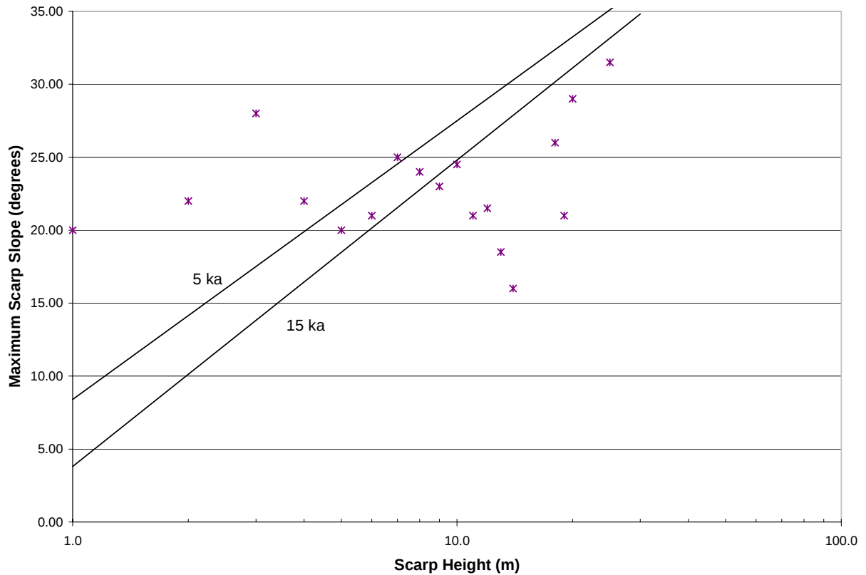
Figure 4.5. Scarp data from the Whitmore Canyon fault scarps. Scarp data straddle the middle Holocene and latest Pleistocene regressions from Machette and McGimsey (1982) and Bucknam and Anderson (1979), respectively.
