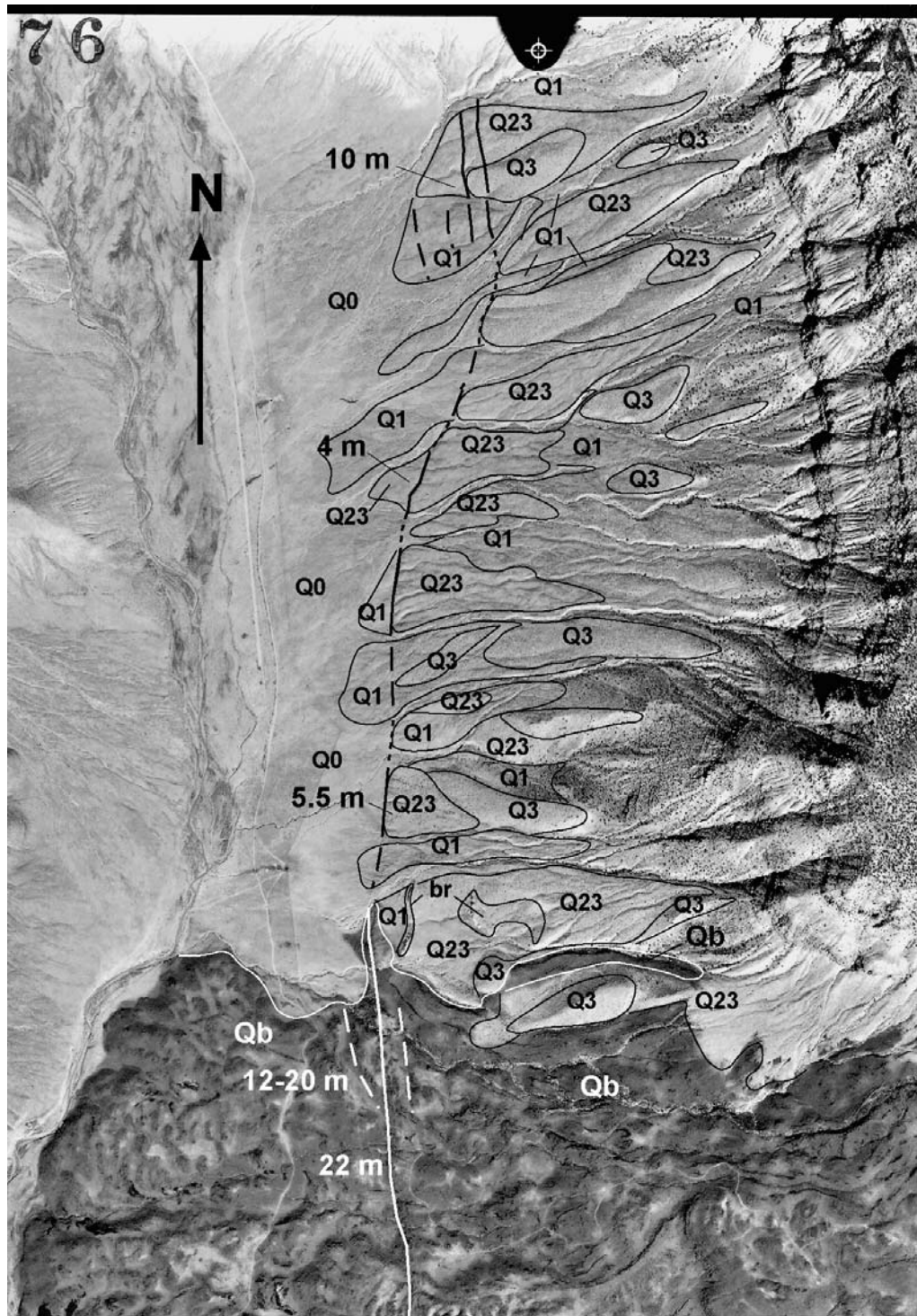
Figure 4.2. Preliminary surficial geologic map along the Hurricane fault in Whitmore Canyon. Map covers most of the north piedmont and the northern part of the Bar Ten basalt flow. The Hurricane fault is shown by bold lines, dashed where uncertain, dotted where concealed beneath young deposits. Surficial geologic units of early Holocene age and older are displaced by the fault (units Q1, Q23, and Q3). Middle to late Holocene fans, terraces, and active channels (unit Q0) are not displaced. Map scale is approximately 1:24,000. Figure modified December 2000.
