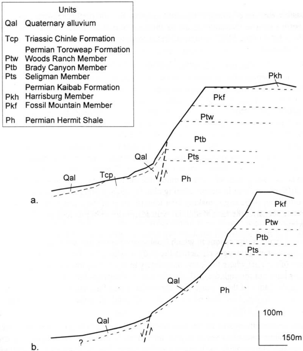
Figure 3.12. Schematic geologic cross-sections across the Hurricane fault illustrating conditions favoring or reducing the chance for preservation of alluvial fault scarps. The Hermit Shale is less resistant to erosion than the Toroweap and Kaibab Formations. In (a) the Hermit Shale does not outcrop and the cliff slope is steeper than in (b) where the Hermit Shale does outcrop. The cliff has eroded farther away from the fault trace in situation (b) and preserves evidence of late Quaternary rupture that may not be preserved in the steeper and bedrock conditions of (a). Surficial unit contacts are from Billingsley (1992); the geology is inferred at depth.
