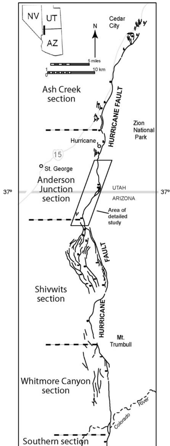
Figure 3.1. Map of the Hurricane fault and the divisions of its five sections. The boxed study area is the site of detailed work and is shown in Fig. 3.2. Fault trace convexities and steps observable here are used in defining section boundaries. Faults mapped by P. Pearthree, 1998.
