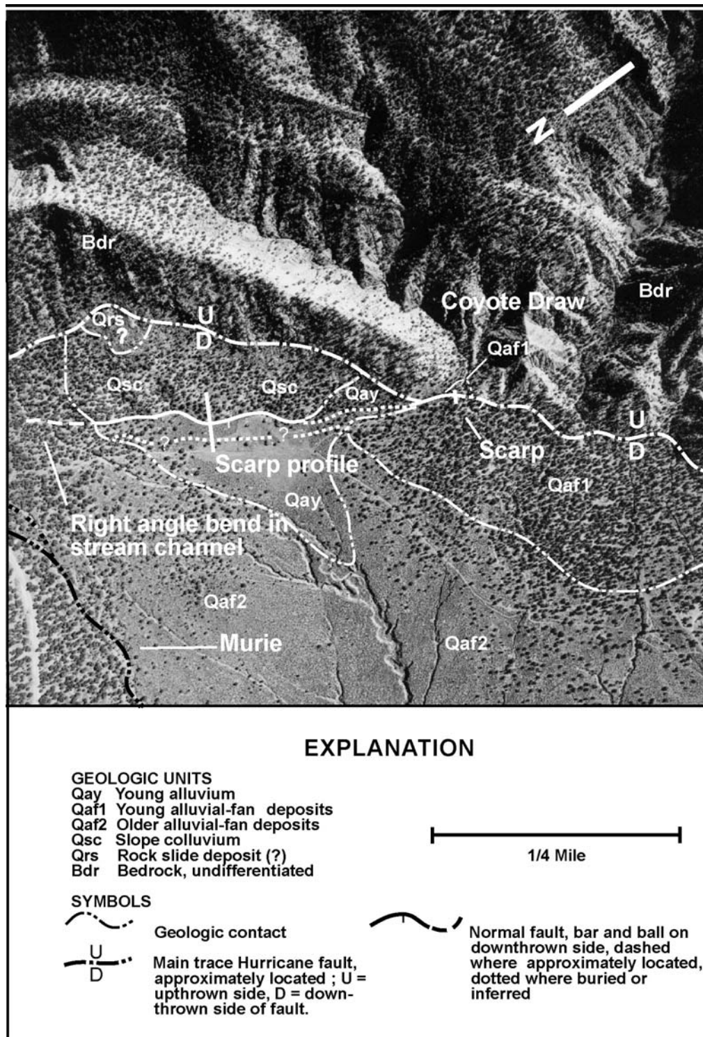
Figure 2.5. Aerial photograph – geologic map of the Murie Creek site, Hurricane fault, Utah.
