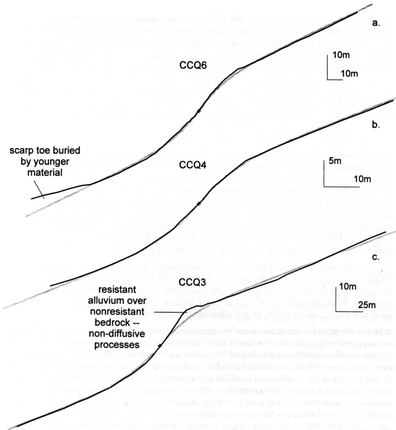
Figure 3.9. Geomorphic models (gray lines) of the Cottonwood Canyon fault scarps (a) CCQ6, (b) CCQ4, and (c) CCQ3 (black lines). Models produced mass diffusivity values of 2-3 \text{m}^2/\text{ky} , 2-4 \text{m}^2/\text{ky} , and 7-12 \text{m}^2/\text{ky} , respectively.
