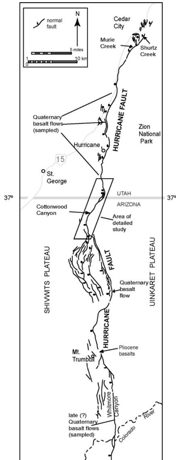
Figure 1.1. Hurricane fault and subsidiary structures in northwestern Arizona and southwestern Utah. Locations of key study sites and basalt flows are shown.
