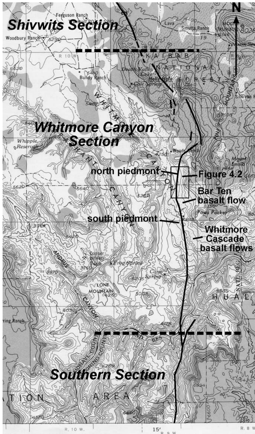
Figure 4.1. Generalized map of the Hurricane fault in Whitmore Canyon. The bold horizontal lines indicate the approximate locations of section boundaries, as defined by Pearthree (1998). The area of Figure 4.2 is shown by the rectangle in Whitmore Canyon, and informal geographic and geologic features are highlighted. Map scale is 1:250,000.
