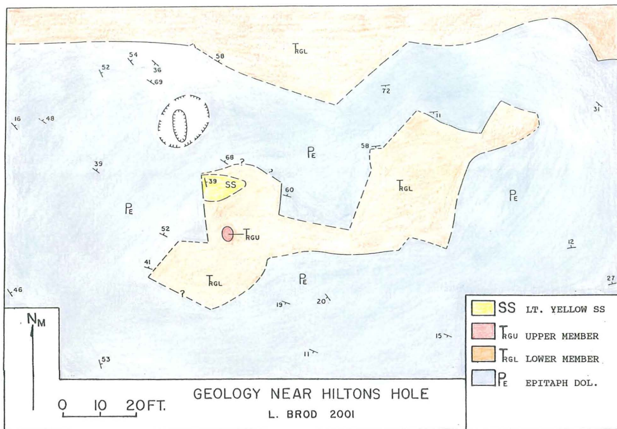
GEOLOGY OF ENLARGED AREA ON HILTON RIDGE FIGURE 8
