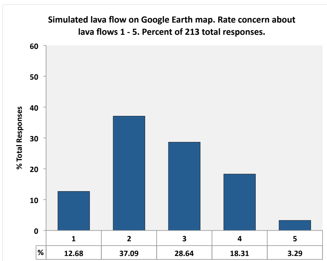
Figure 4.4. Level of Concern for Method C. This method included the example lava flow on Google Earth. Participants were asked to rate their concern from 1 (not concerned at all) to 5 (very concerned).
